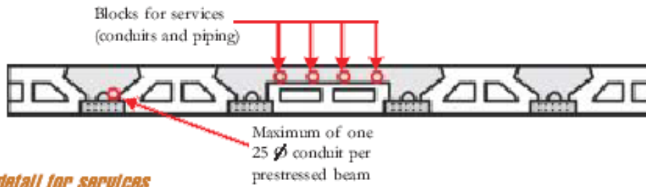
Slab detail for services
